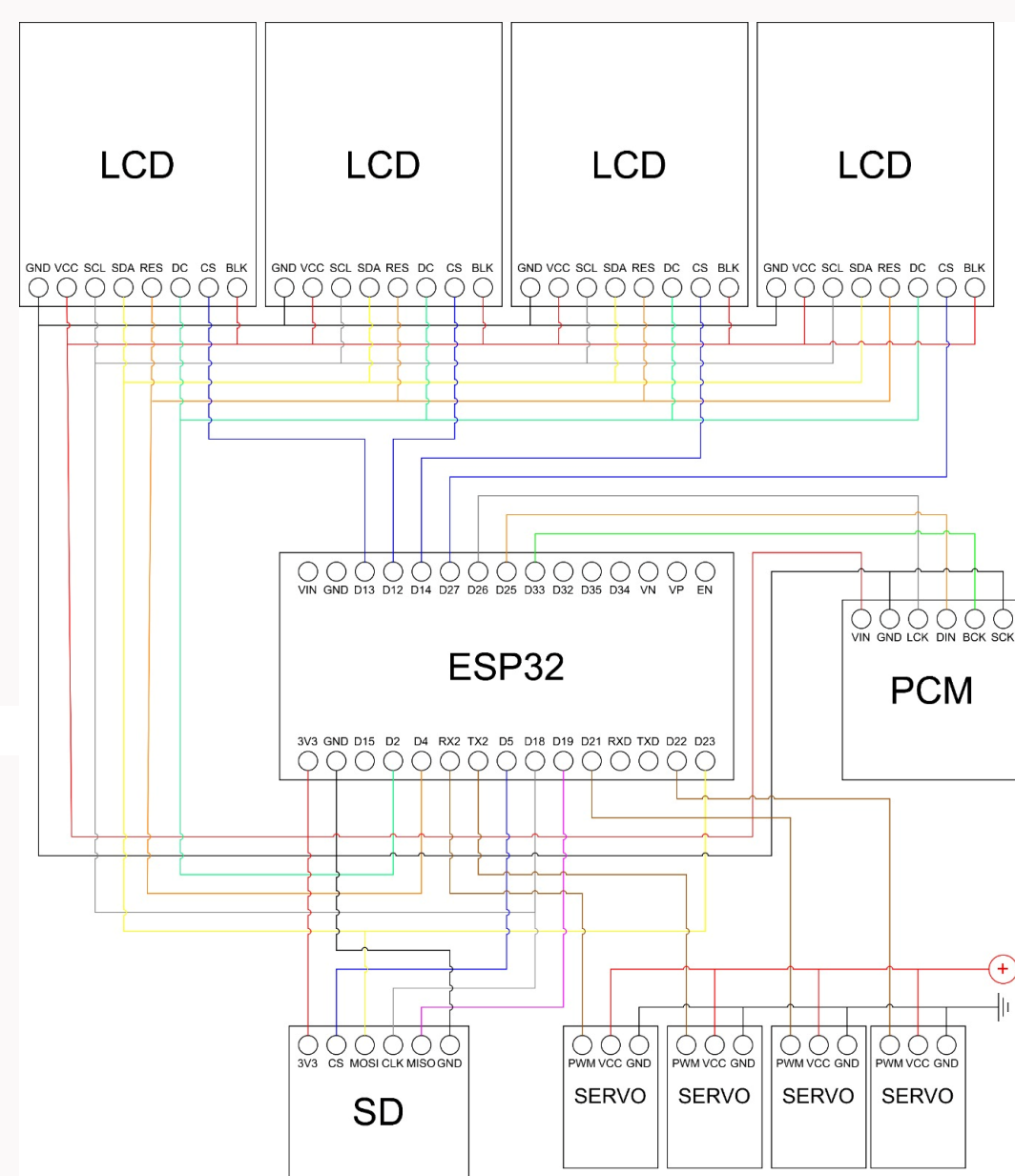
Wiring diagram
